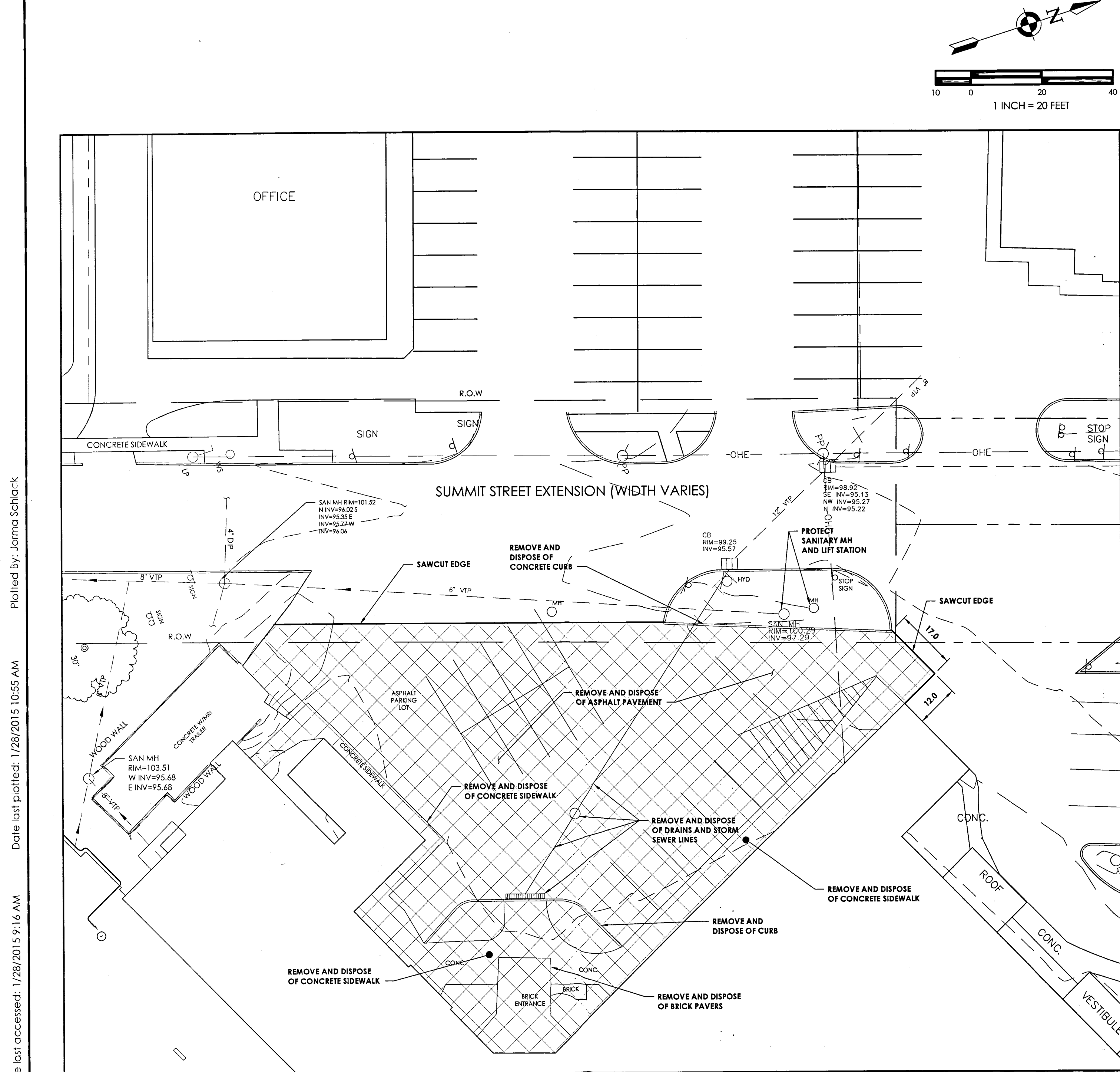
DEMOLITION PLAN
