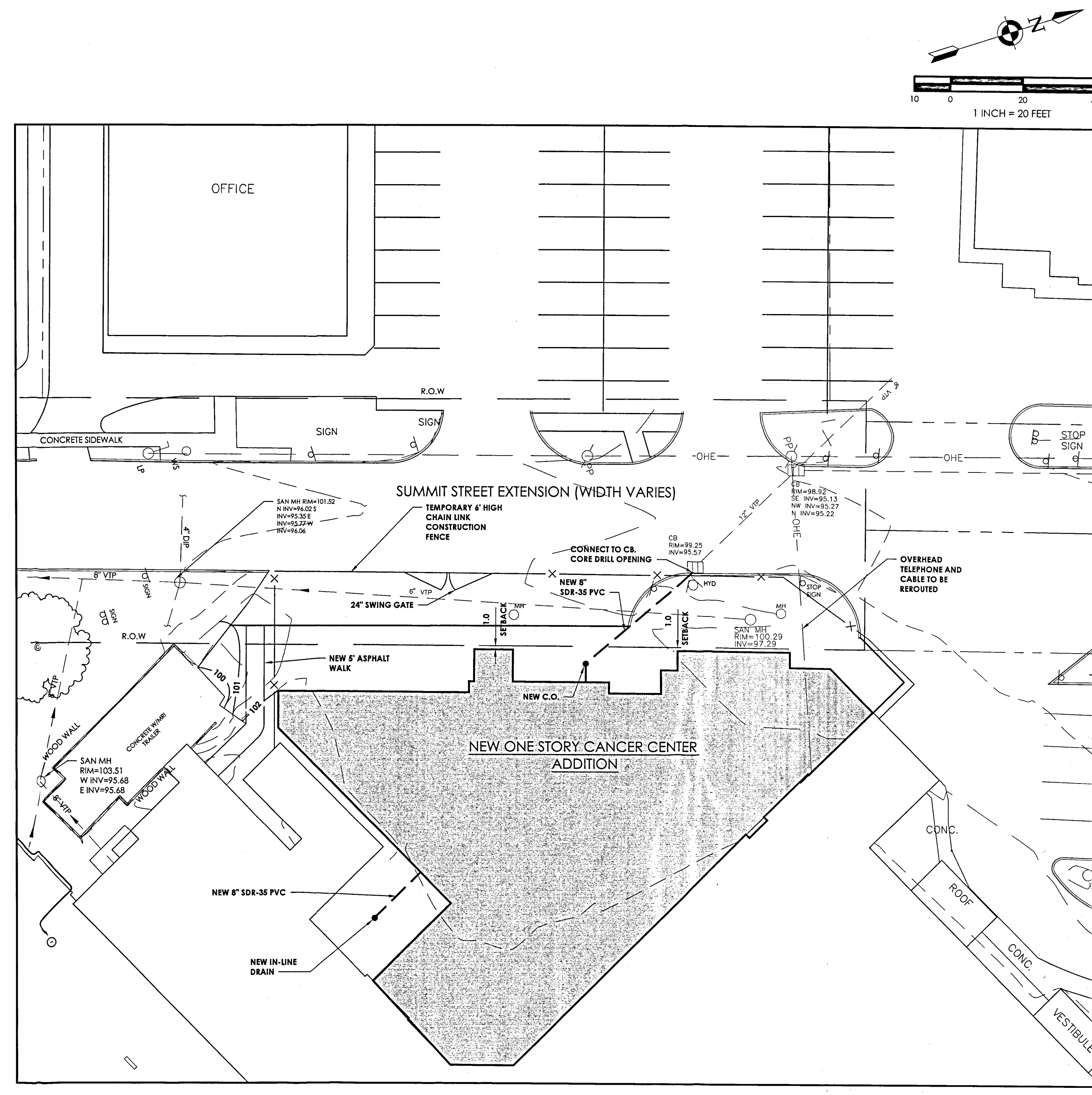
SITE PLAN
